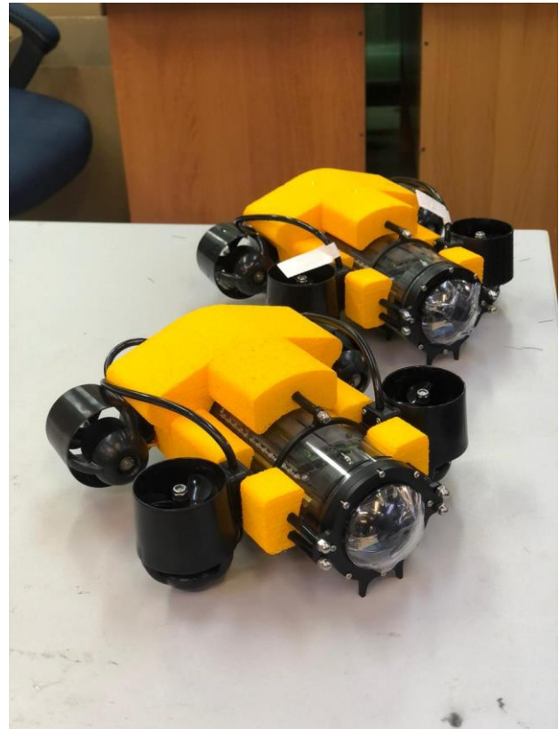
Fig. 2. MiddleAUVs
